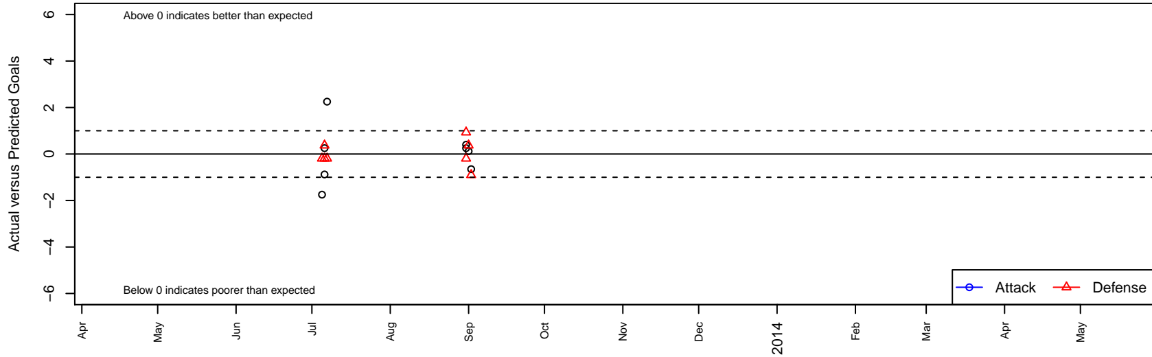
WPFC Fury Black B94 Dots are actual minus expected GF (blue circles) and GA (red triangles). Blue line is smoothed change in attack strength. Red is smoothed change in defense strength.
